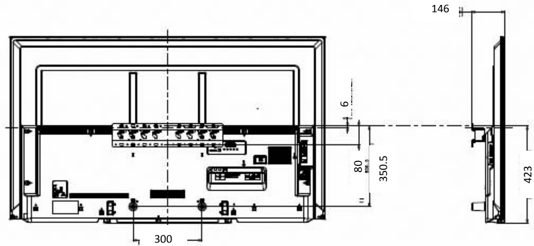
SU-WL450 (STANDARD)
